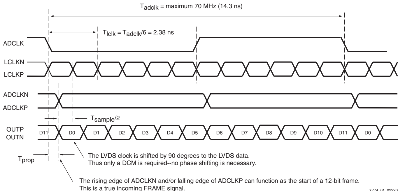
Figure 1: LVDS Timing Diagram (One Channel)
