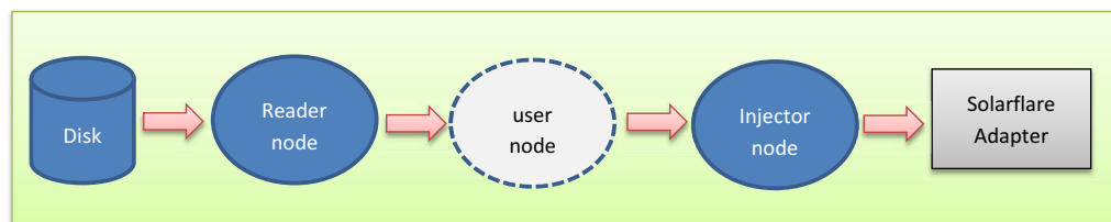
Figure 8: SolarReplay Sequence
